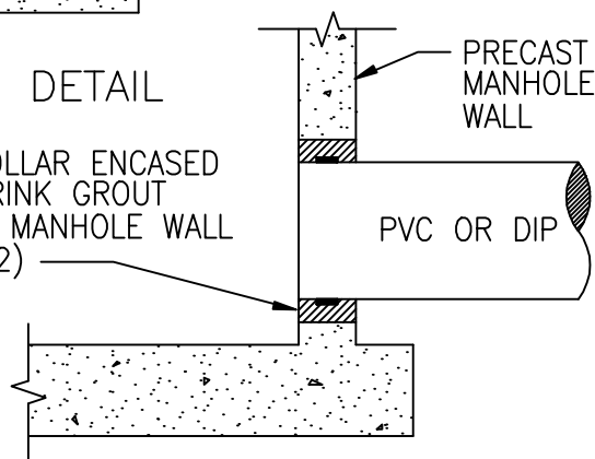
SPECIAL DETAIL FOR 24" DIAMETER PIPE AND LARGER
