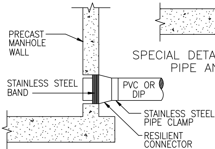
STANDARD PRECAST MANHOLE PIPE CONNECTION
